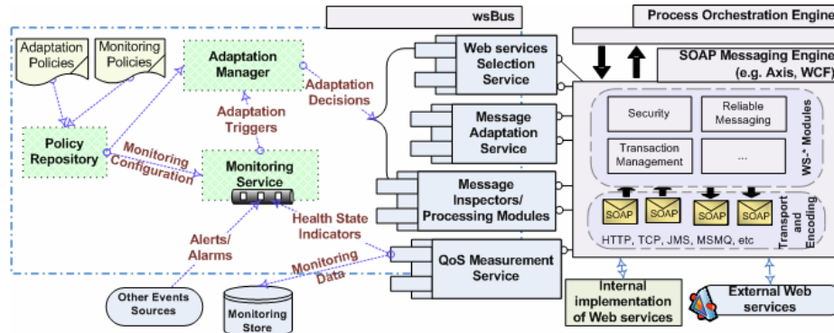
Fig. 3. wsBus Architecture
