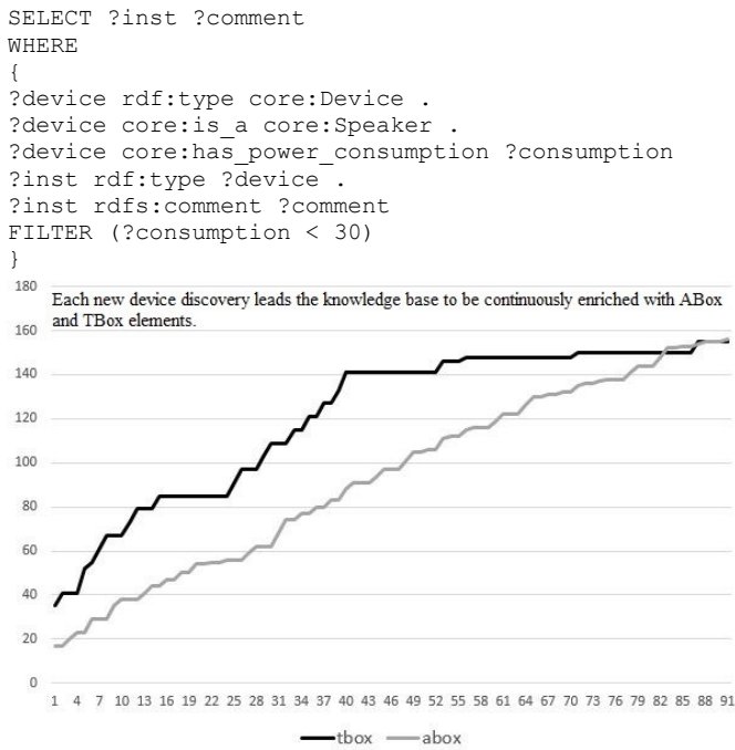
Fig. 5. Devices discovery: ABox/TBox enrichment
