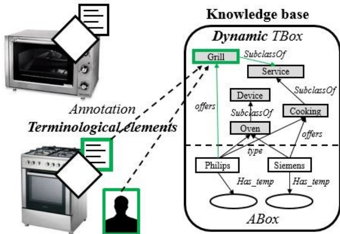
Fig. 3. The terminological dynamicity level
